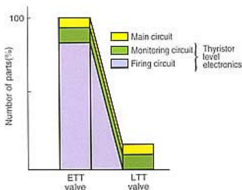
Figure 4 Number of parts in a valve
