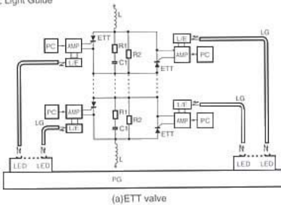
(a)ETT valve
