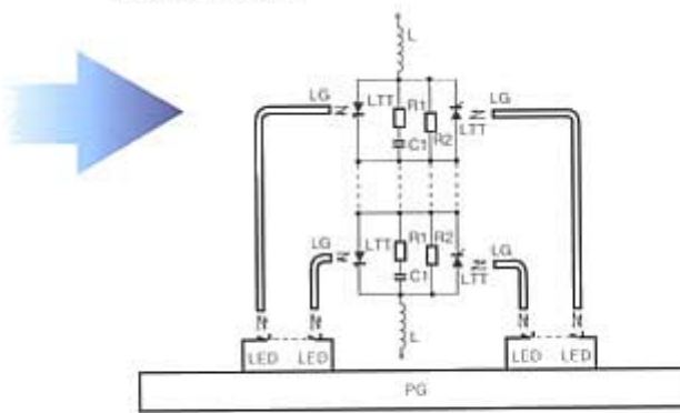
(b)LTT valve
