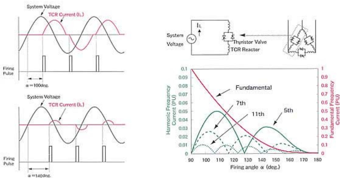
Figure 2 TCR Current and firing angle
