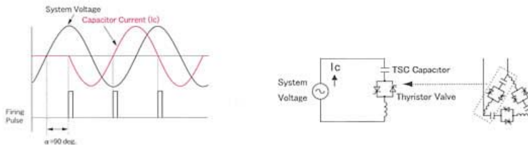
Figure 3 TSC Current and firing angle
