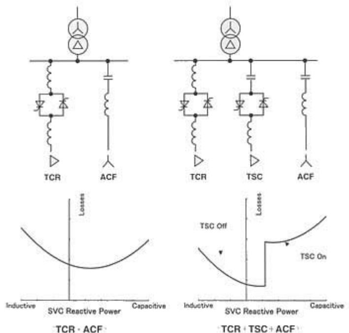
Figure 1 Typical Configuration of SVC
