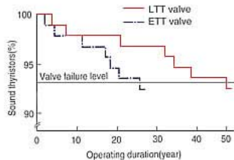
Figure 5 Reliability Comparison of valves
