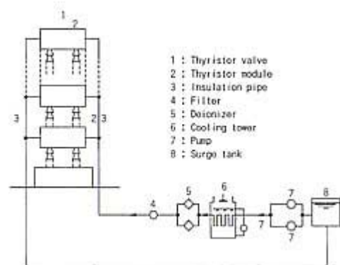
Figure 6 Valve (Water) Cooling System
